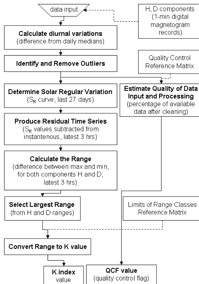
Fig.4. Schematic of the algorithm for real-time calculation of the K index.
