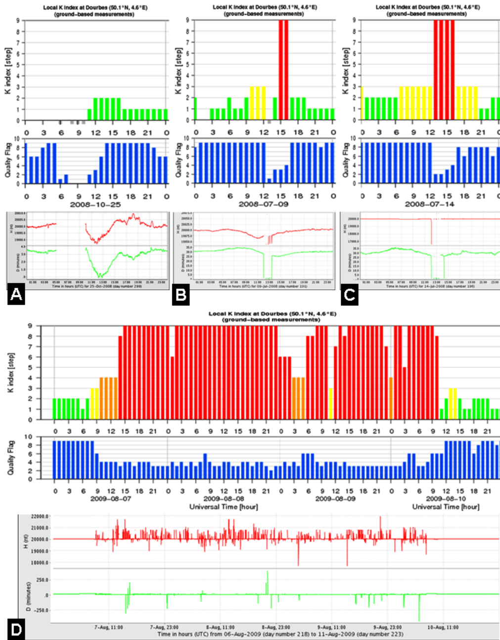
Fig.9. Nowcast system's handling spurious/noisy data and technicalities.
