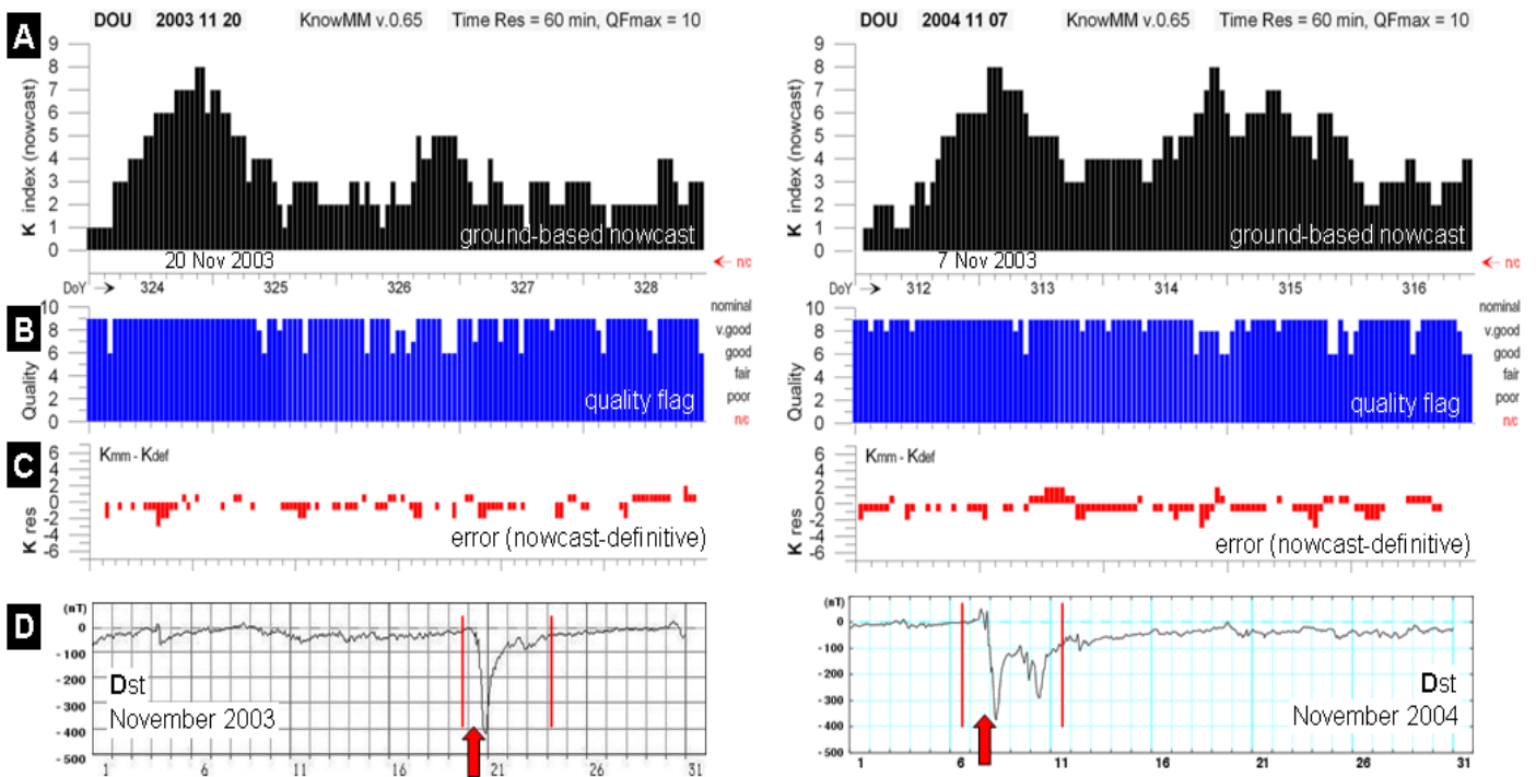
Fig.11. Evaluation results of the K index operational production during the major storm events in November 2003 and 2004. Panel (A): K index nowcast. (B): Quality flag. (C): Residual errors, nowcast (Kest) minus definitive (Kdef) values. (D): Dst index.
