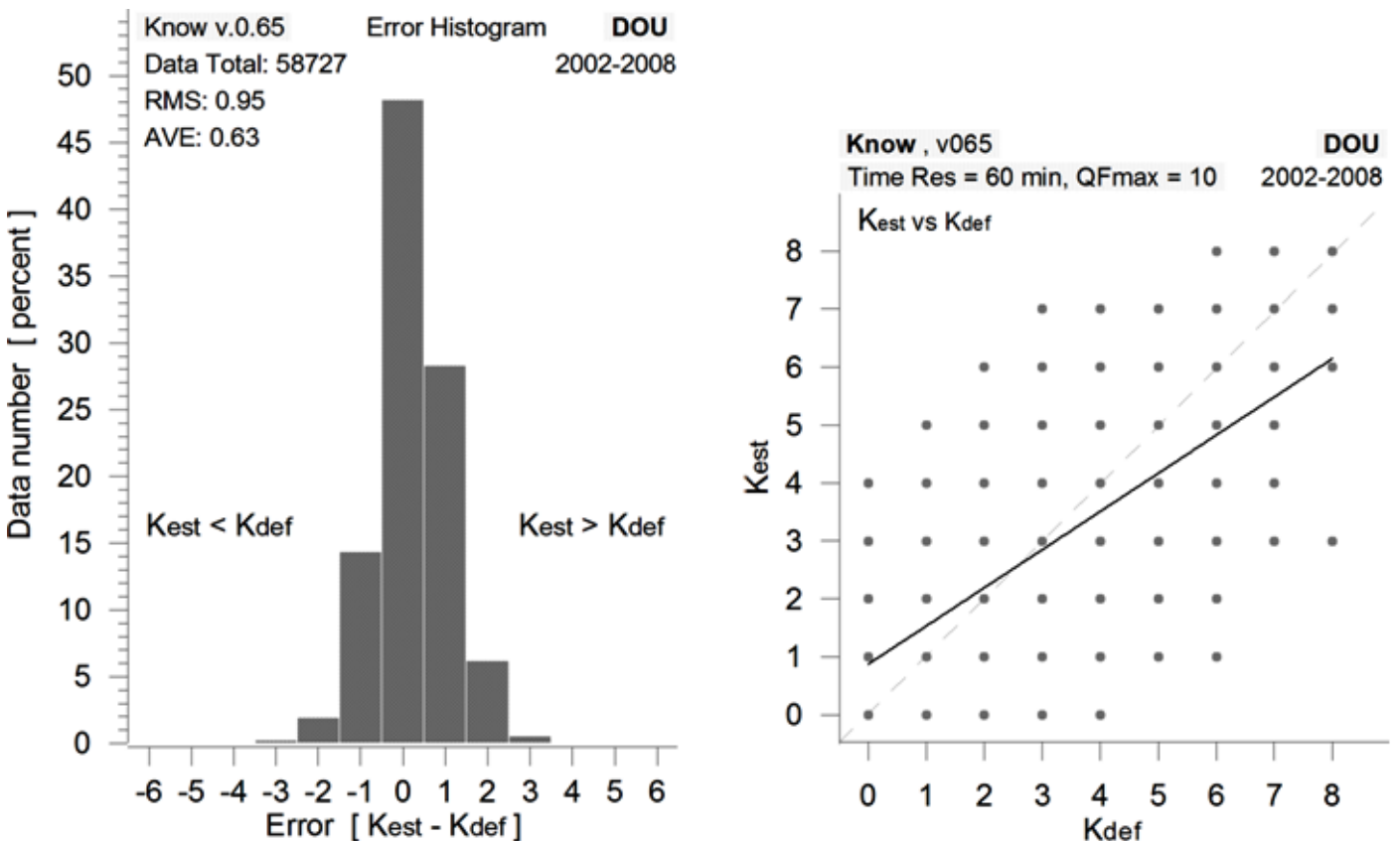
Fig.12. Evaluation results of the K index nowcast production over the period of 2002-2008. Left: Histogram of the residual errors, nowcast K ( K_{est} ) minus definitive K ( K_{def} ). Right: Scatter plot of nowcast K vs definitive K values.
