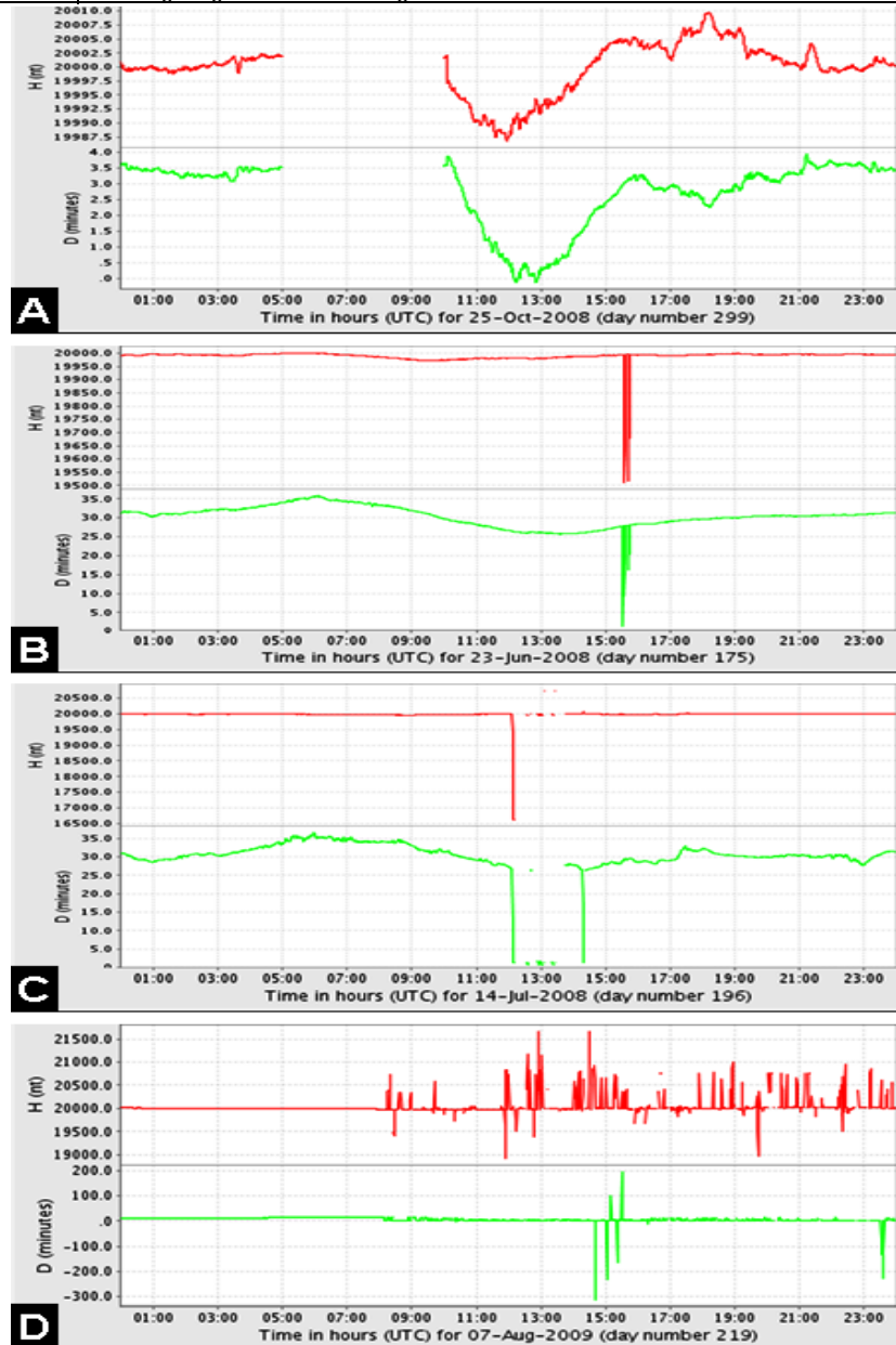
Fig.5. Identification of gaps and spurious/noisy data. Panel (A): Data gap. (B): Cluster of outliers. (C): Data gap accompanied with outliers and regular data. (D): Sustained occurrence of noisy data due to technical problems.
