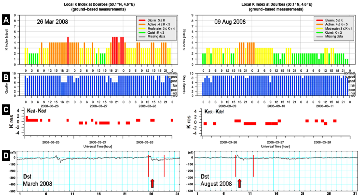
Fig.10. Exemplary results of K index operational production during recent minor geomagnetic events of increased geomagnetic activity. Panel (A): K index nowcast. (B): Quality flag. (C): Residual errors, nowcast (Kest) minus definitive (Kdef) values. (D): Dst index, for reference only.
