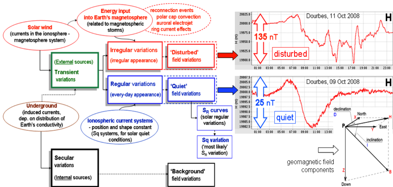
Fig.1. Geomagnetic field components and variations – secular/transient, regular/irregular and quiet/disturbed (after Menvielle and Berthelier, 1991; Siebert, 1996 ).
