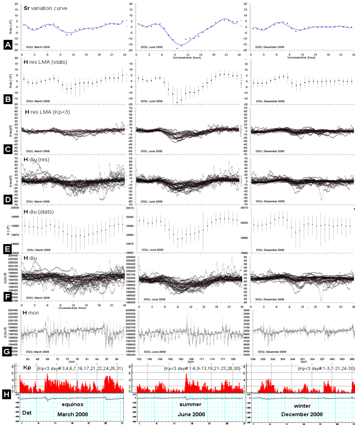
Fig.6. The S_R curve establishment from 1-min measurements of the H component from observations at Dourbes during equinox (left panels), summer (middle), and winter (right) months. Bottom panel (H) shows the global geomagnetic activity as described by the Kp and Dst indices. (G): Real-time 1-min measurements of the H component. (F): The superposed diurnal variations. (E): Median (solid circles), mean (—) and standard deviations (vertical bars) of the diurnal variations. (D): Diurnal variations (relative) with daily medians removed. (C): Diurnal variations (relative, cleaned) from quiet days ( K_p < 3 ) only. (B): Median (solid circles), mean (—) and standard deviations (vertical bars) of the diurnal variations (relative, quiet-days). (A): The S_R curve (polynomial approximation) based on the median diurnal relative quiet-day variations.
