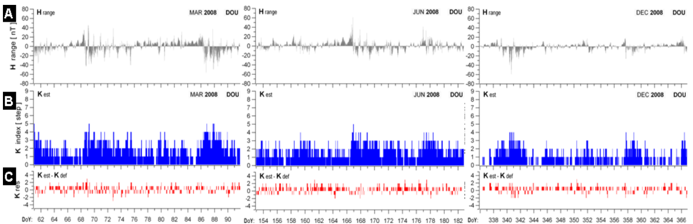
Fig.7. Results of the K index nowcast (panels B) together with the corresponding residual errors, i.e. nowcast minus definitive values (panels C) for the months of March, June, and December 2008 as produced from the observations at Dourbes. The top panels (A) display the observed H component's deviations from the S_R curve.
