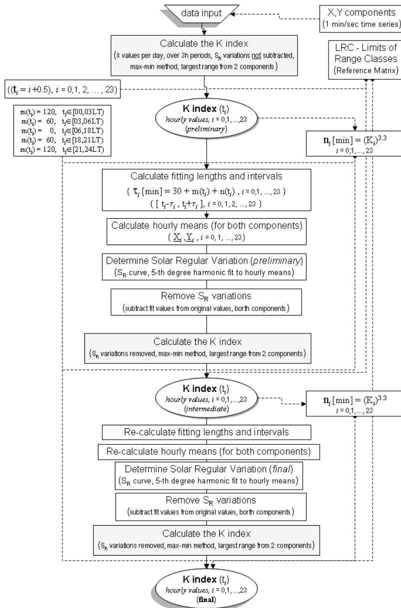
Fig.3. The K index calculation based on the linear elimination algorithm (after Sucksdorff et al., 1991 ).
