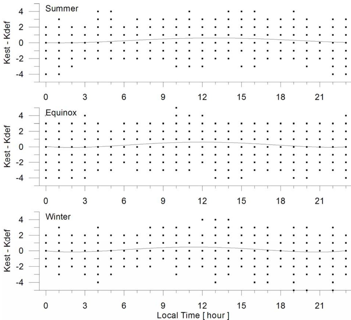
Fig.13. Evaluation results of the K index nowcast for the period of years 2002-2008, Dourbes. Seasonal and local time variations of the difference between the nowcast K (Kest) and definitive K (Kdef) values.
