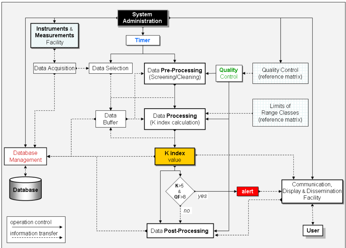
Fig.8. The K index nowcast/alert system layout.
