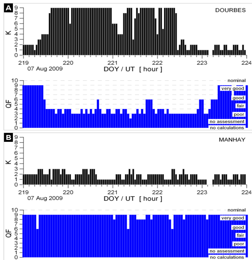
Fig.14. Comparison between the K index calculations at two observatories in a close distance, Dourbes (panel A) and Manhay (panel B).
